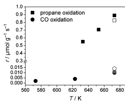
Figure 15. Rates of consumption of propane and CO over a polycrystalline complex oxide catalyst (MoVNbTeO 4-x ; M1 phase). The molar ratio of the reactants in the feed for the oxidation of propane corresponds to C 3 H 8 /O 2 /H 2 O/N 2 = 3:6:40:51 vol%. The measurements were performed at a contact time of 0.81 g(cat.) s mL -1 (filled squares). A different M1 batch was measured only at 673 K and a contact time of 0.80 g(cat.) s mL -1 (open square). CO oxidation was performed using the latter batch at a contact time of 1.2 g(cat.) s mL -1 in dry feed composed of CO/O 2 /H 2 O/N 2 = 3:6:0:91 vol% (black circles). Decreasing the contact time to 0.80 g(cat.) s mL -1 at 673 K results in only slightly increased rate of CO consumption in the dry feed (gray circle) and in the presence of 40 vol% steam (CO/O 2 /H 2 O/N 2 = 3:6:40:51, open circle).
