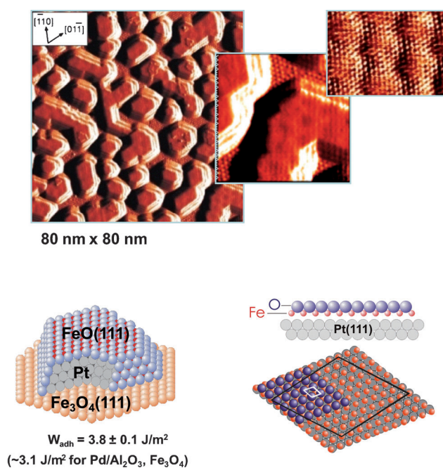
Figure 13. Scanning tunneling images of Pt nanoparticles supported on a Fe 3 O 4 (111) film grown on Pt(111) (the magnetite film thickness represents the bulk) after heating to 850 K. [131,132] Schematic representation of the formed FeO-encapsulated Pt nanoparticles together with the mark of adhesion determined by a Wulff–Kaichev analysis compared to those determined in the same way for Pd supported on different substrates. [132,138] Schematic representation of the double-layer FeO film grown on Pt(111) together with the determined structural parameters. [134,135]
