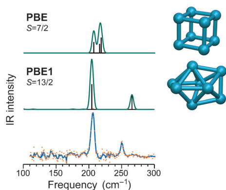
Figure 2. Experimental far-IR spectrum of \text{Rh}_8^+ (bottom) compared to the predicted IR spectra for the global minimum structures obtained using either a pure functional (PBE) or by including exact exchange with a hybrid functional (PBE1). (From Ref. [45].)
