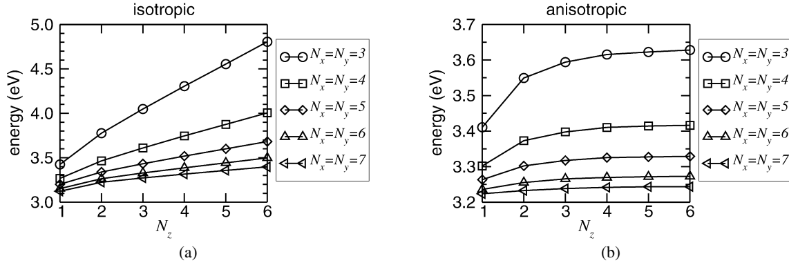
Fig. 1. Convergence of the lowest conduction-band energy with respect to the number of \mathbf{k} -points N_z perpendicular to the surface for (a) the original isotropic implementation and (b) with the anisotropy taken into account. The quantitative behaviour depends on the sampling in the parallel direction ( N_x = N_y ). Note the different scales of the two graphs.
