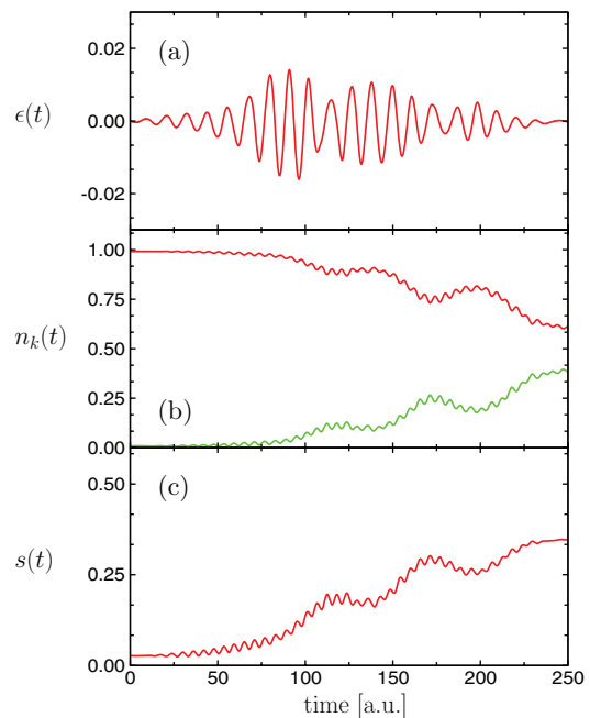
Fig. 2: (Colour on-line) (a) Optimal laser pulse for the transition of the Helium atom from the ground state to the first excited singlet state. The overlap of the propagated wave function and the target state was 98.59% after 12 OCT iterations. (b) The two largest occupation numbers and (c) the correlation entropy as a function of time.
