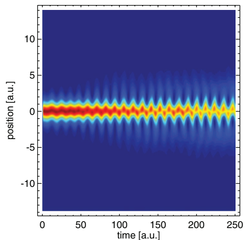
Fig. 3: (Colour on-line) Time evolution of the orbital density of the first natural orbital of helium during the excitation from the ground state to the first excited state. The quiver motion of the electrons is nicely reflected in the density profile of the natural orbital.
