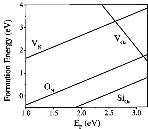
Fig. 1. Formation energy versus Fermi energy for native defects (nitrogen and gallium vacancies) and donors (oxygen and silicon) in GaN. The zero of Fermi energy is located at the top of the valence band.
