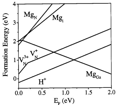
Fig. 2. Formation energy as a function of Fermi level for Mg in different configurations (Ga-substitutional, N-substitutional, and interstitial configuration). Also included are the native defects and interstitial H.
