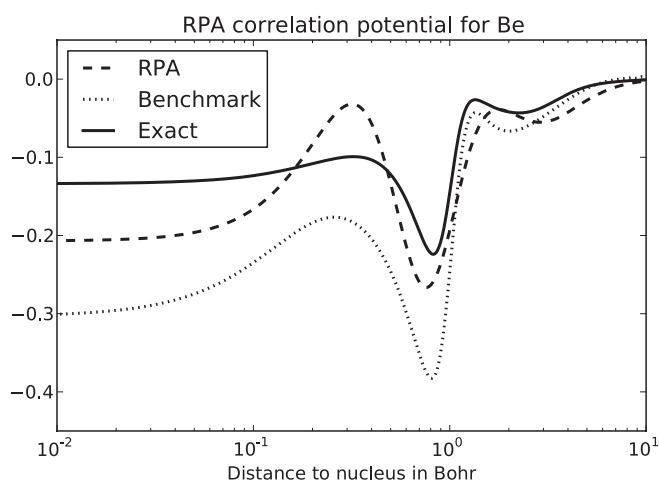
FIG. 2. The correlation potential of Be for RPA (Ref. 38) (dotted), for RPA in this work (dashed), and the exact correlation potential 52 (solid).
