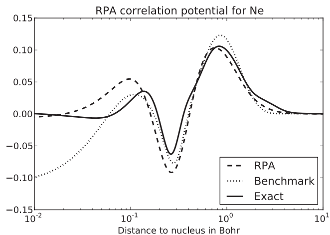
FIG. 3. The correlation potential of Ne for RPA (Ref. 38) (dotted), for RPA in this work (dashed), and the exact correlation potential 52 (solid).
