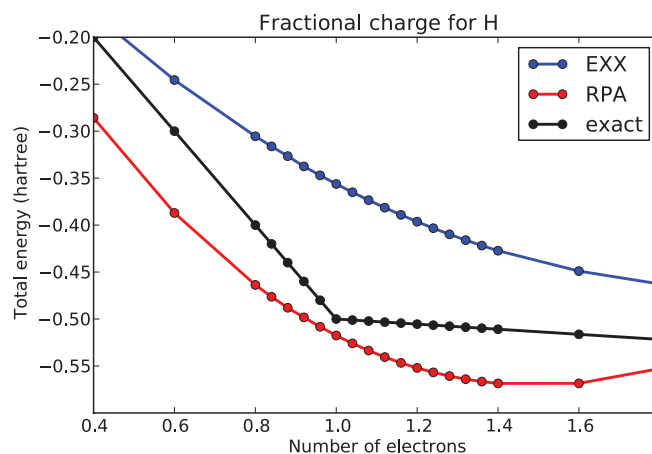
FIG. 8. The total energy of H as a function of number of electrons for EXX (blue), RPA (red), and exact (black).
