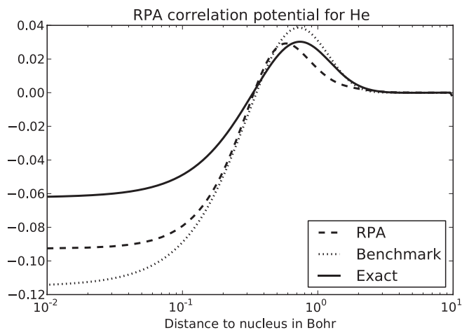
FIG. 1. The correlation potential of He for RPA (Ref. 38) (dotted), for RPA in this work (dashed), and the exact correlation potential 52 (solid).
