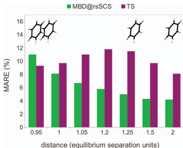
FIG. 2. The mean absolute relative error of PBE0+MBD@rsSCS and PBE0+TS (in %) at each of the S66 \times 7 inter-fragment separations.
