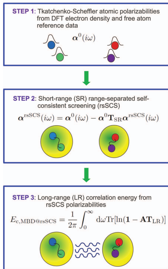
FIG. 1. Schematic diagram illustrating the computation of the MBD@rsSCS long-range correlation energy. Note that in the last term on the right-hand side of the equation in Step 2 all quantities are \omega dependent.
