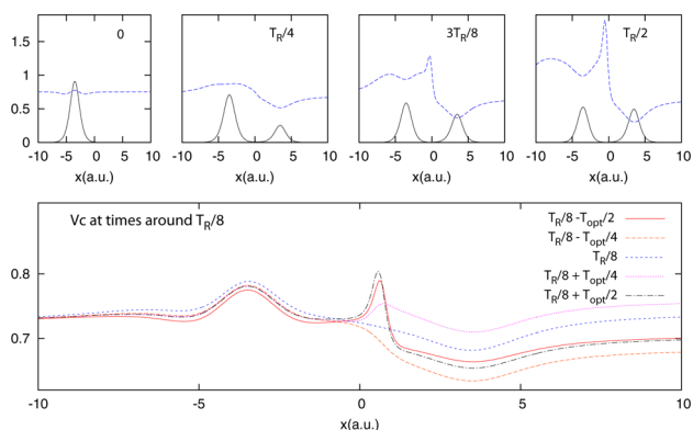
Figure 3. (Upper panel) The correlation potential (dotted blue line) and density (solid black) shown at snapshots of time indicated. (Lower panel) V_C snapshots over an optical cycle centered at around T_R/8 .
