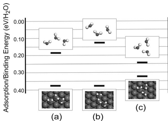
Fig. 2 Relative energies and structures of three gas phase and adsorbed H 2 O trimers. Adsorption energies and binding energies are relative to isolated gas phase H 2 O molecules as defined in eqn (1) and (2), respectively.
