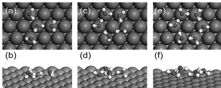
Fig. 3 Top and side views of the lowest energy structures identified for an adsorbed H 2 O tetramer ((a)–(b)), pentamer ((c)–(d)), and hexamer ((e)–(f)) on Cu(111).
