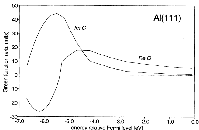
FIG. 3. Energy dependence of -\text{Im}G_{AA}^+ at a tip-sample separation of 4.3 \text{ \AA} with the tip above an Al atom.
