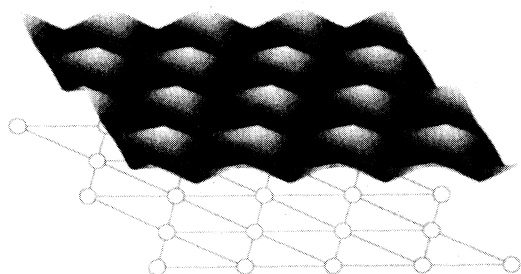
FIG. 4. Lateral variation of the capacitor projected local density at the Fermi level (CAP-LOD) [cf. Eq. (8)] for Al(111) at a tip-sample separation of 4.3 \text{ \AA} .
