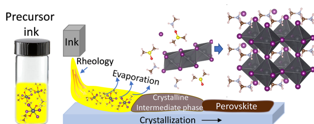
FIG. 14. Schematic representation of the role of solvent in the transformation of hybrid perovskite precursor solution into a thin film. Adapted with permission from Shargaieva et al. , Mater. Adv. 1 , 3314 (2020). Copyright 2020 The Royal Society of Chemistry.
