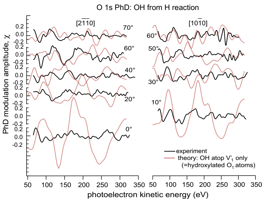
Fig. 6. Comparison of the experimental O 1s (OH) PhD spectra from the H-dosed V_2O_3(0001) surface with the results of multiple-scattering calculations assuming the hydroxylated emitter O atoms are atop the outermost layer V'_1 atoms (equivalent to hydroxylated vanadyl O_1 atoms, see Fig. 4b).
