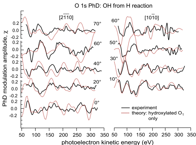
Fig. 7. Comparison of the experimental O 1s (OH) PhD spectra from the H-dosed V_2O_3(0001) surface with the results of multiple-scattering calculations assuming the emitter atoms are hydroxylated O_1 atoms (see Figs. 1 and 4c).
