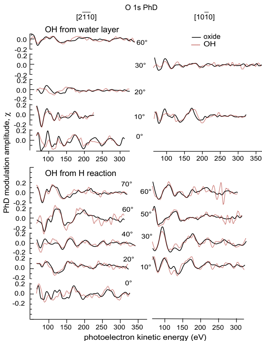
Fig. 5. Comparison of the experimental PhD spectra recorded from the OH and oxide components of the O 1s emission, from OH-covered surfaces prepared by the two alternative methods, in a range of different emission geometries as specified by the azimuth and polar angle.
