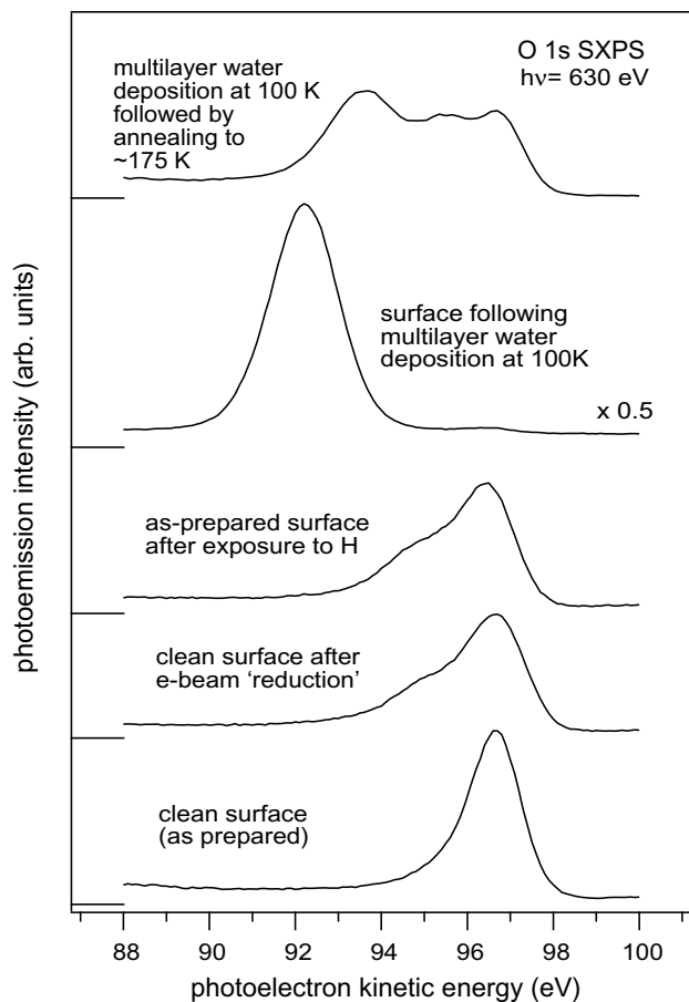
Fig. 2. Typical SXPS spectra showing the O 1s emission peak region for different surface treatments of the V_2O_5(0001) film, recorded at a photon energy of 630 eV and a polar emission angle of 60^\circ . The spectra are displaced in intensity as shown by the offset zero lines on the left.
