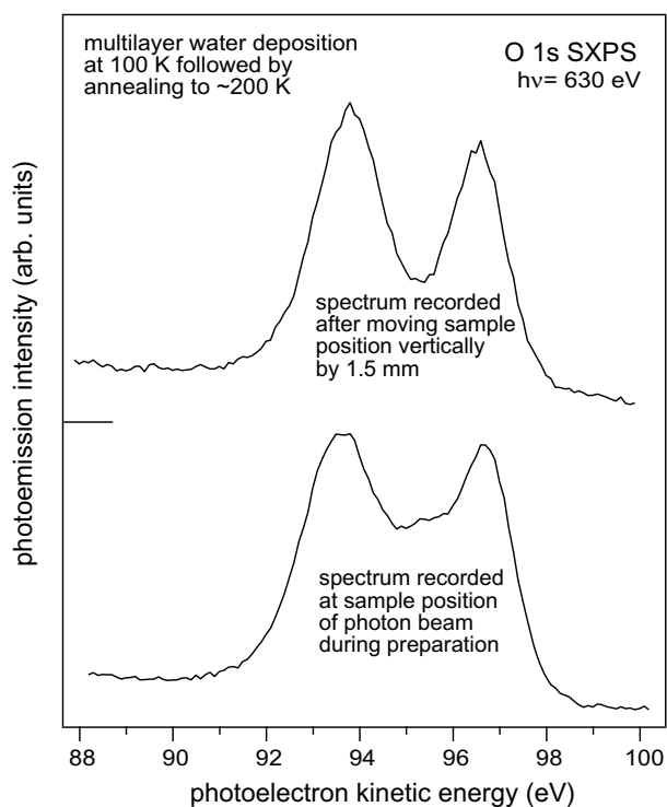
Fig. 3. SXPS spectra showing the O 1s emission peak region from a V_2O_3(0001) surface covered with a water multilayer at \sim 100 K and then heated to \sim 200 K. The lower spectrum was recorded in normal emission with the sample fixed in position following monitoring of the deposition and heating sequence by photoemission. The upper spectrum was recorded after moving the sample by 1.5 mm so that the incidence flux of 630 eV photons hit a different part of the sample.
