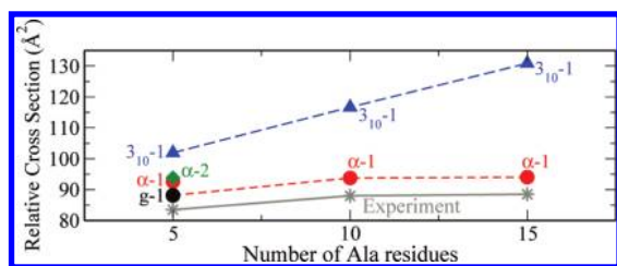
Figure 3. Ac-Ala n -LysH + , n = 5,10,15: Calculated (using an empirical rare gas–molecule interaction potential 34 ) ion-mobility cross sections and comparison with experiment (ref 8). Blue triangles correspond to conformers in the 3_{10-1} geometry, red circles correspond to conformers in the \alpha -1 geometry, the black circle corresponds to the g -1 conformer, the green diamond corresponds to the \alpha -2 conformer, and gray stars correspond to the experimental data from ref 8. The solid and dashed lines serve only as a guide to the eye, and have no physical significance.
